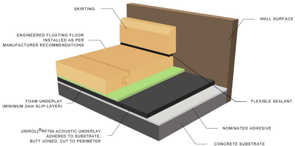
FLOATING TIMBER FLOORING SYSTEM.
