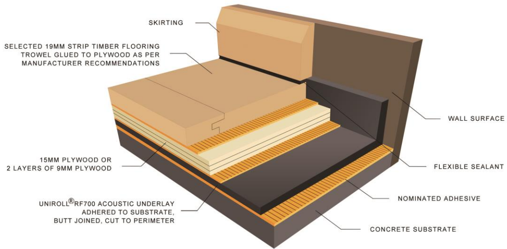
STRIP TIMBER FLOORING SYSTEM
