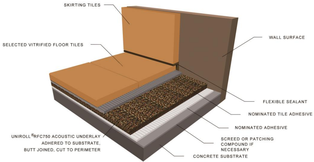
DIRECT STICK SYSTEM
