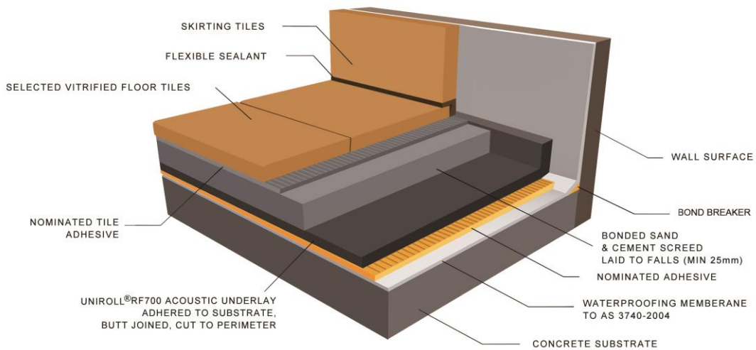
UNDER SCREED SYSTEM
